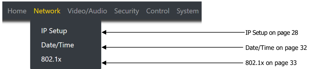
FIG. 17 Network Page
