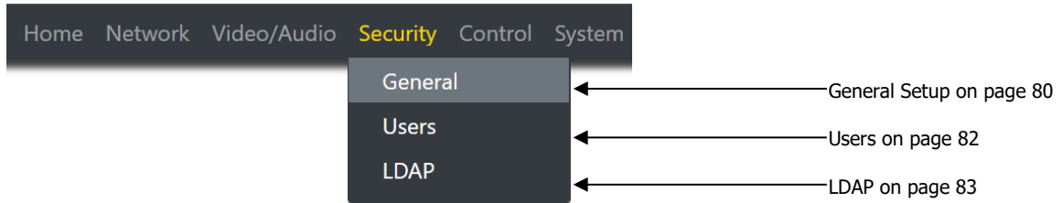
FIG. 66 Security Page
