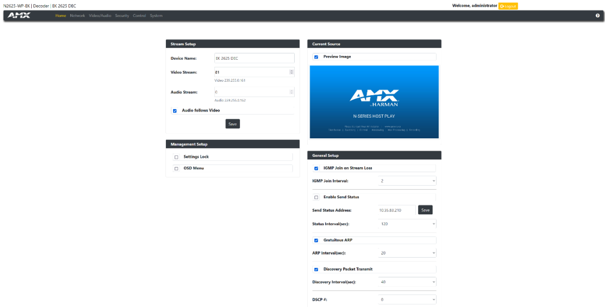
FIG. 45 Settings Page
