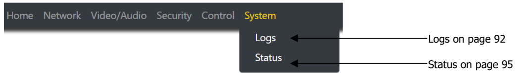
FIG. 78 System Page
