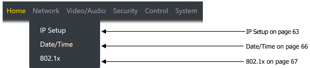
FIG. 50 Network Page
