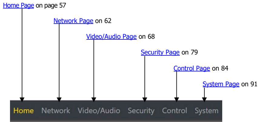
FIG. 44 Section Links
